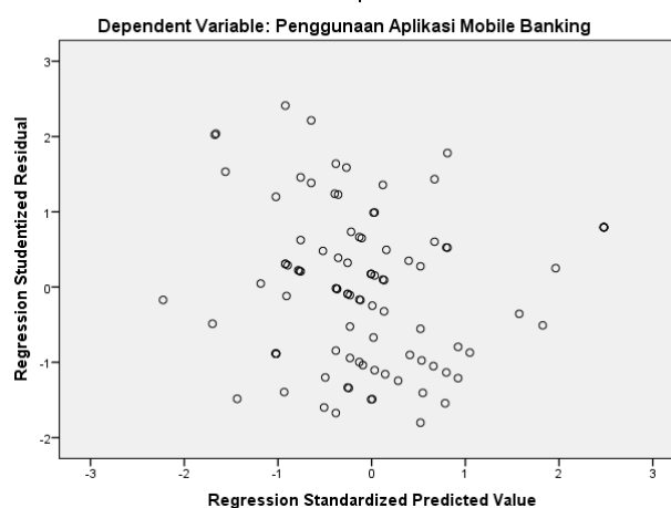
Gambar 3.4 Uji Heteroskedastisitas Scatterplot
