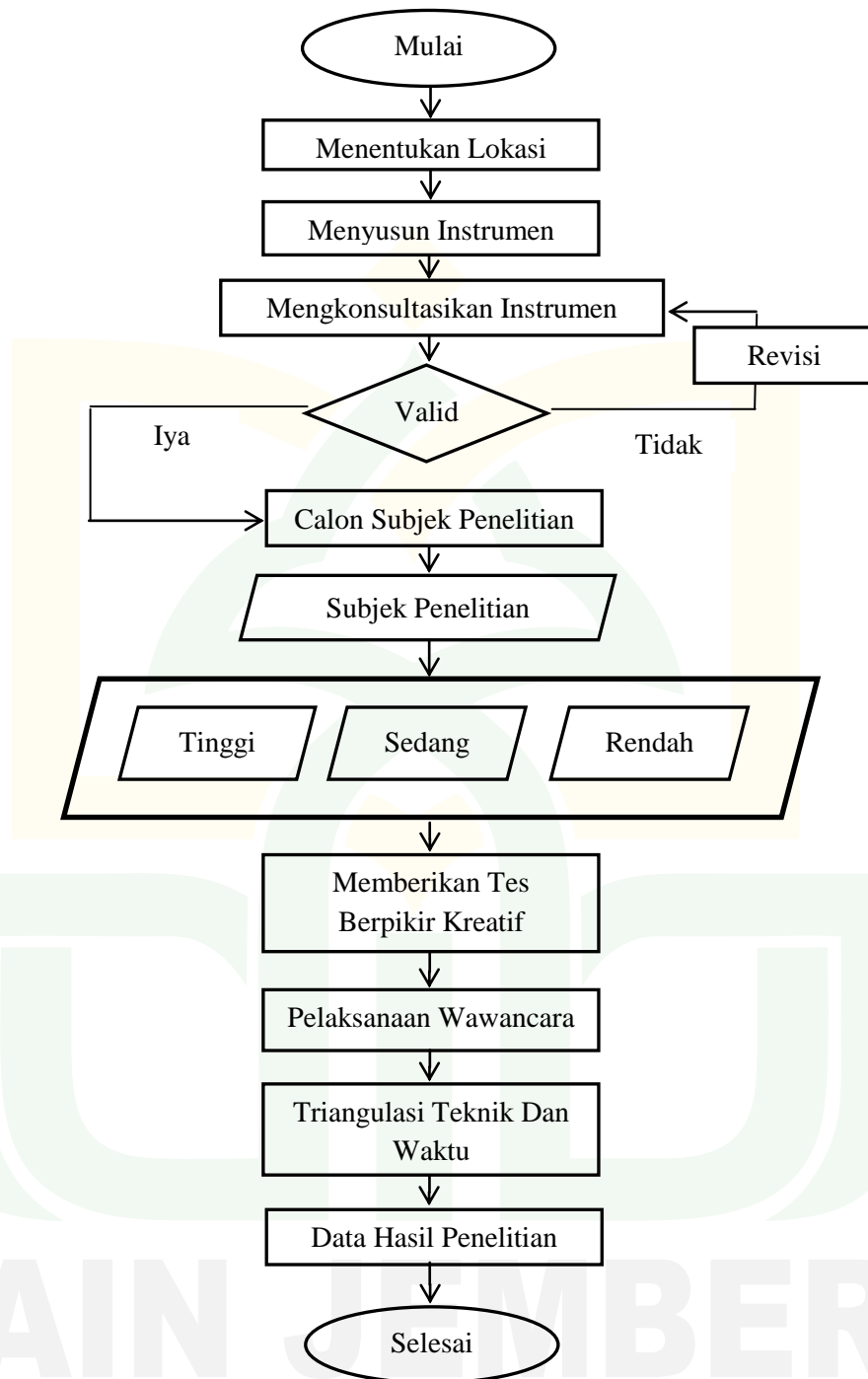
Gambar 3.2 Alur Penelitian
